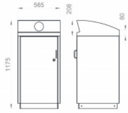
Curved Recycling (304SSCR)
