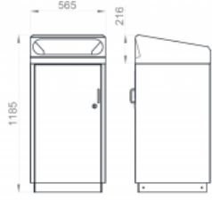
Tapered Frontry (304SSTF or MSTF)
