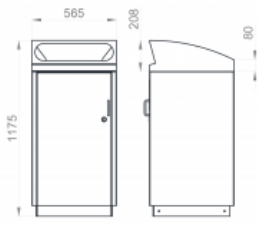
Curved Litter (304SSCL)
