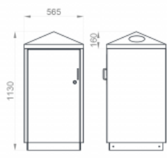
High Pyramid Recycling (304SSRH)
