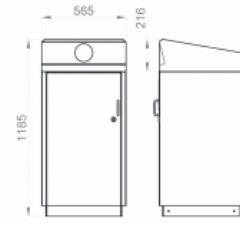
Tapered Recycling (304SSTR or MSTR)
