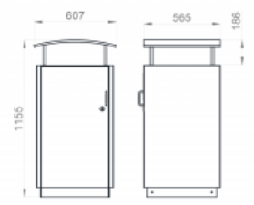
Flat with Canopy (304SSFC)
