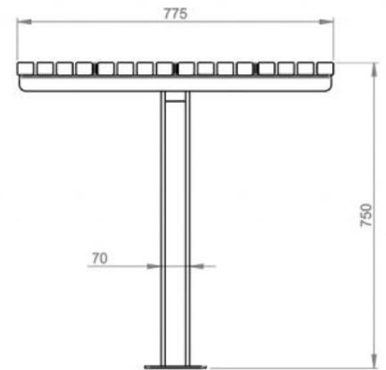
RIGHT VIEW
