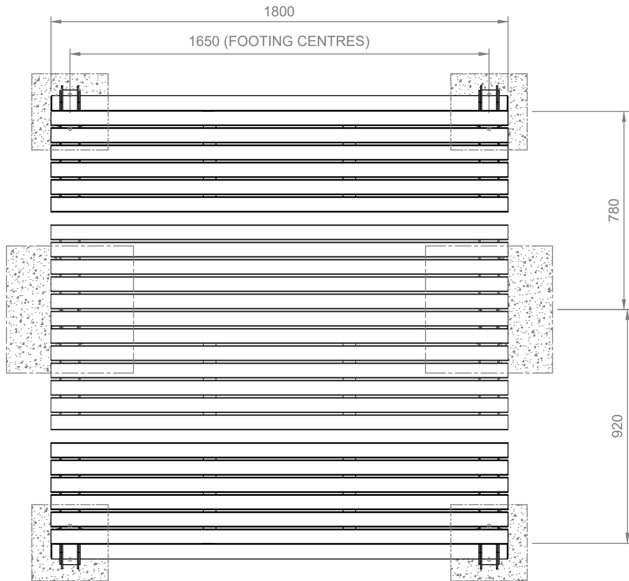
Top View
