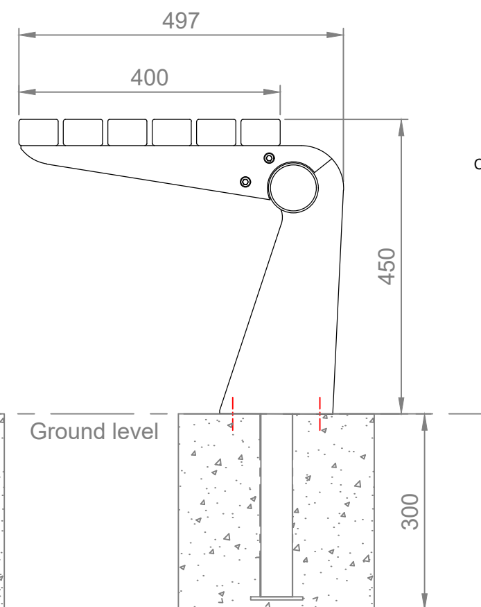
Right View
