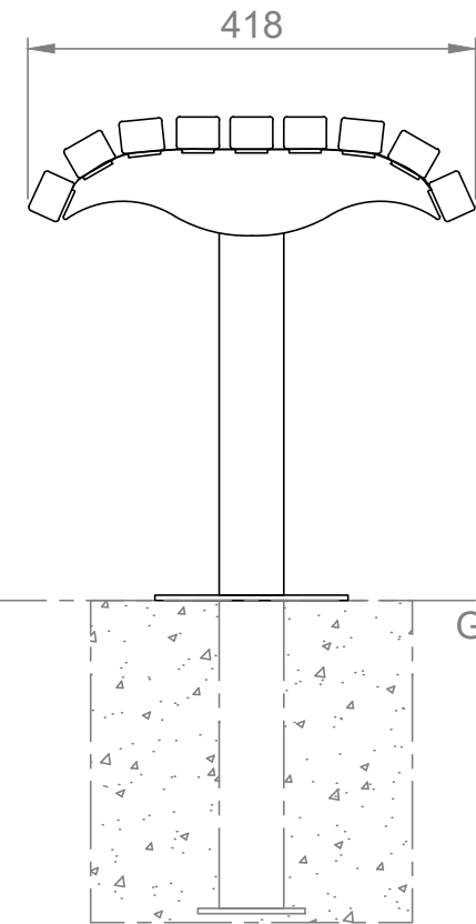
End View
